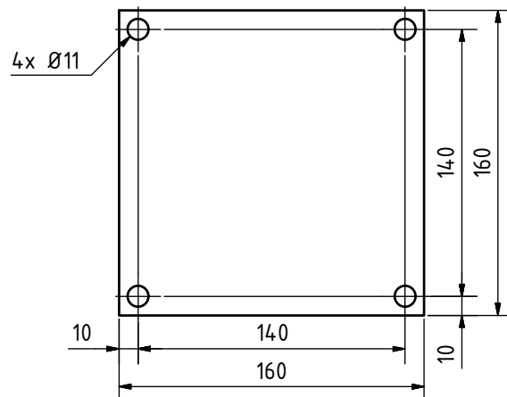
Bodenplatte/ground plate
